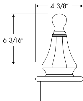
4" DIAMETER POST TENON
