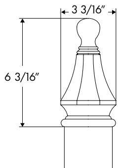
3" DIAMETER POST TENON
