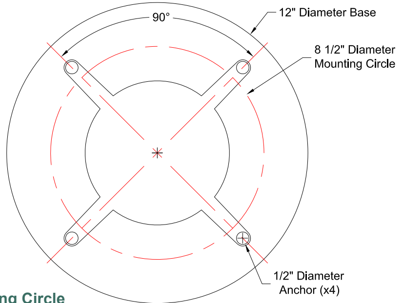
Mounting Circle
