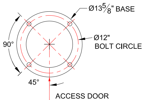
MOUNTING DETAIL
